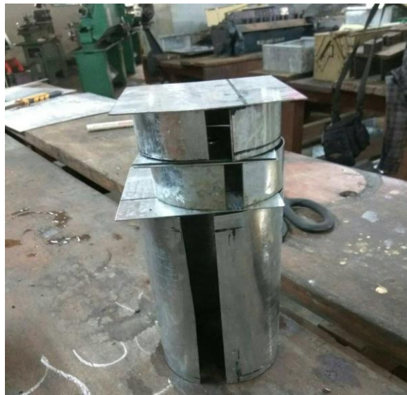
Gambar 2. Rangka cyclone
