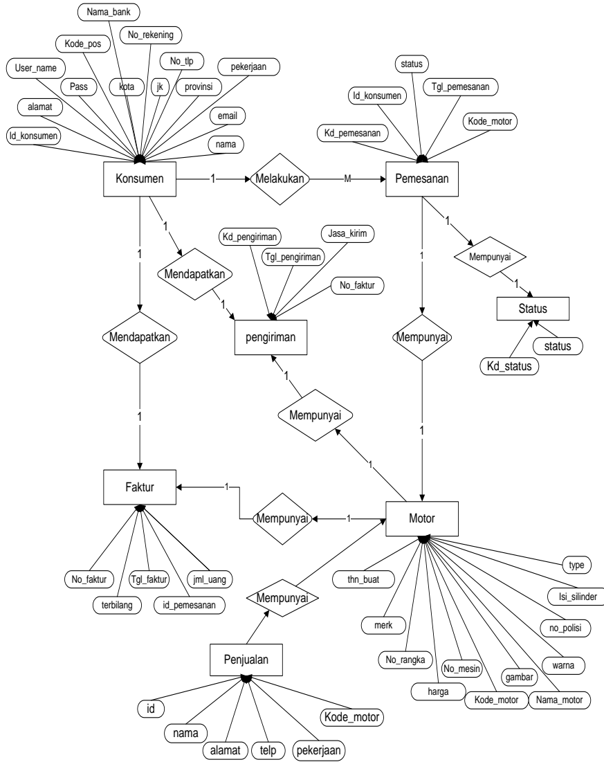
Gambar 3. Entity Relational Diagram (ERD)
